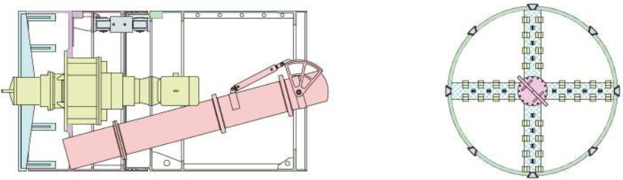
浓泥加压系列(适用卵石地层) CONCENTRATED MUD PRESSURE SERIES (FOR PEBBLES& GRAVEL LAYER)
